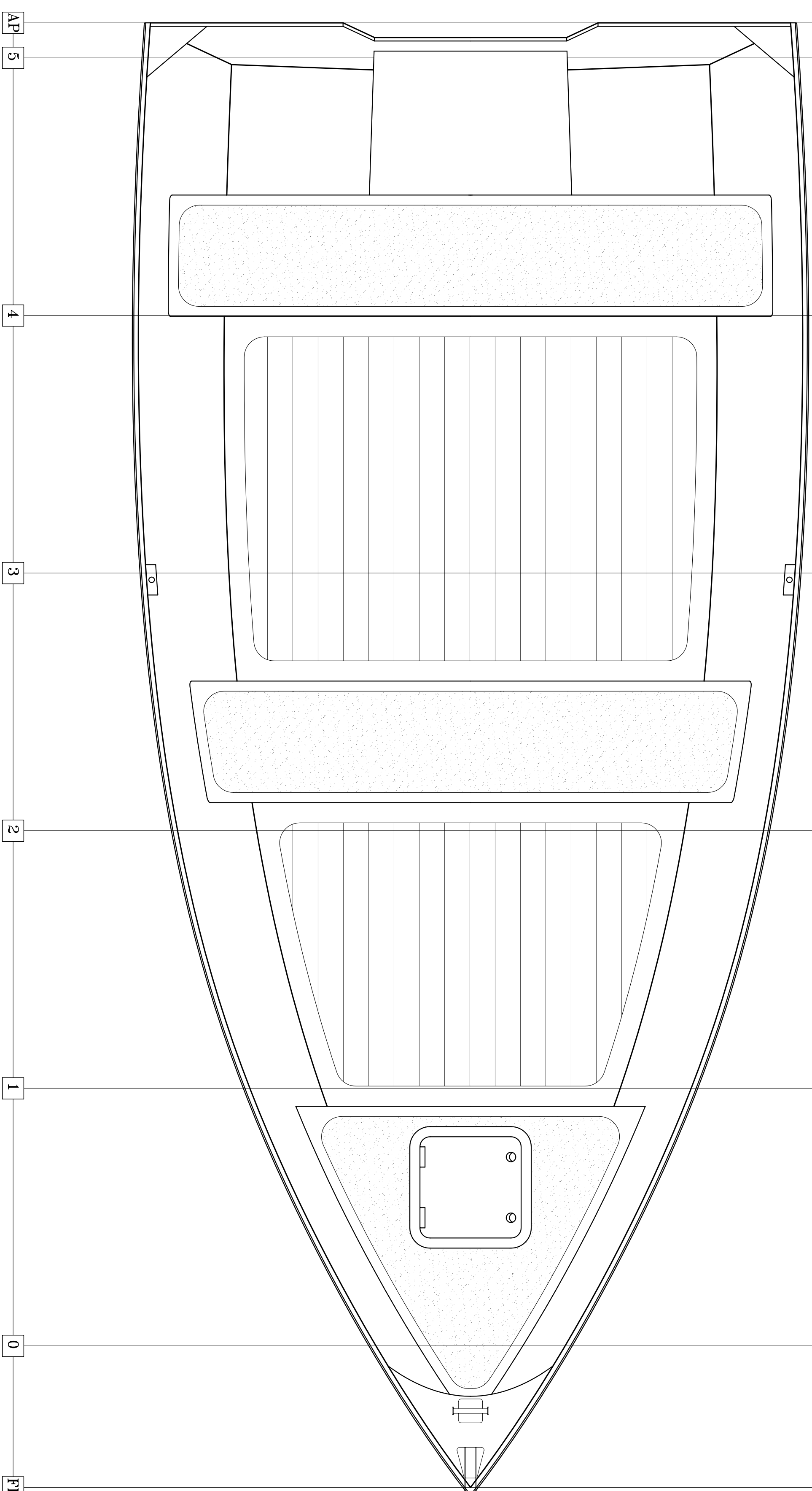
PLAN VIEW
