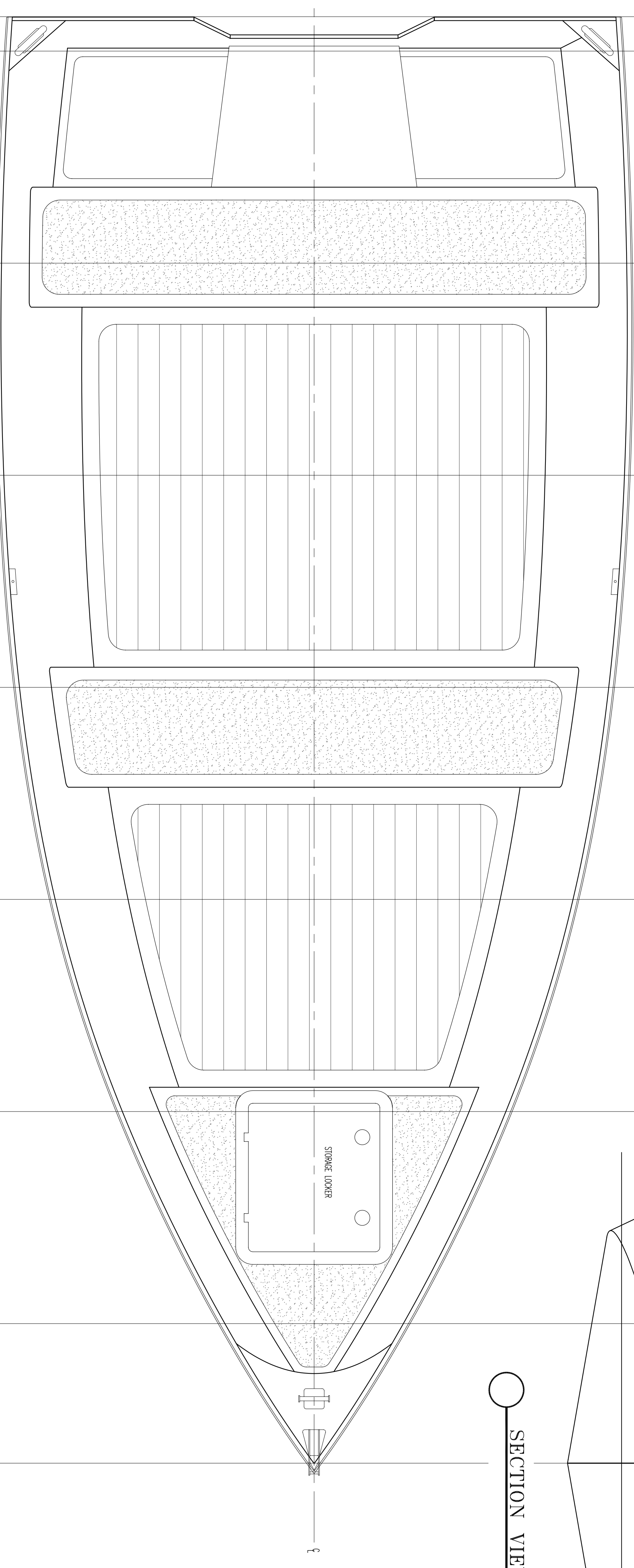
○ PLAN VIEW
